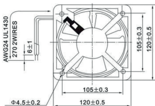
Outline drawing
